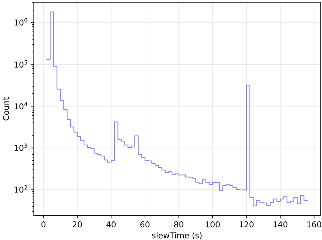
too_elab_r16_d3_griz_v3.4_10yrs All visits: Slew Time Histogram
