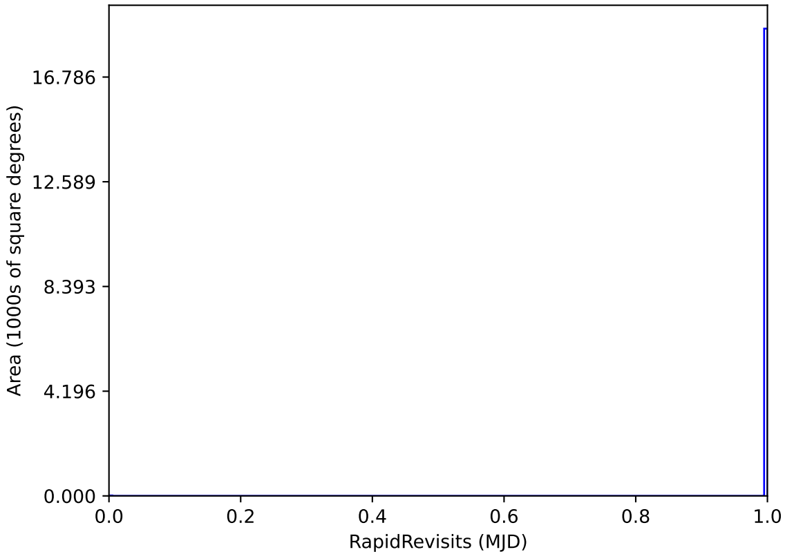
too_elab_r16_d3_griz_v3.4_10yrs WFD: RapidRevisits
