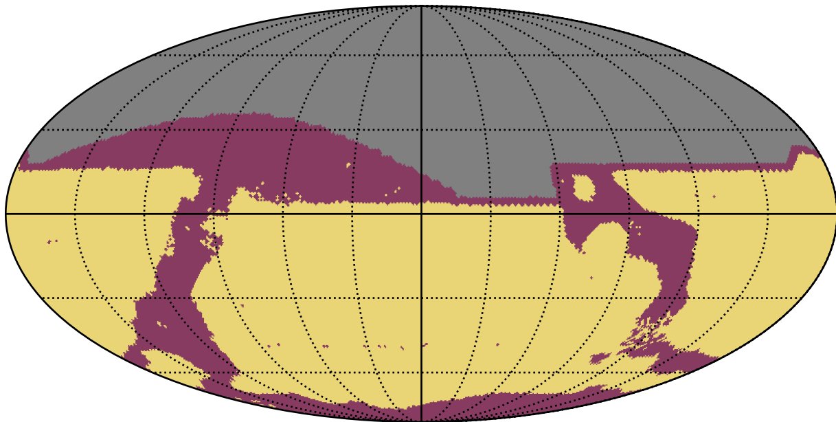
too_elab_r16_d3_griz_v3.4_10yrs All sky: RapidRevisits
