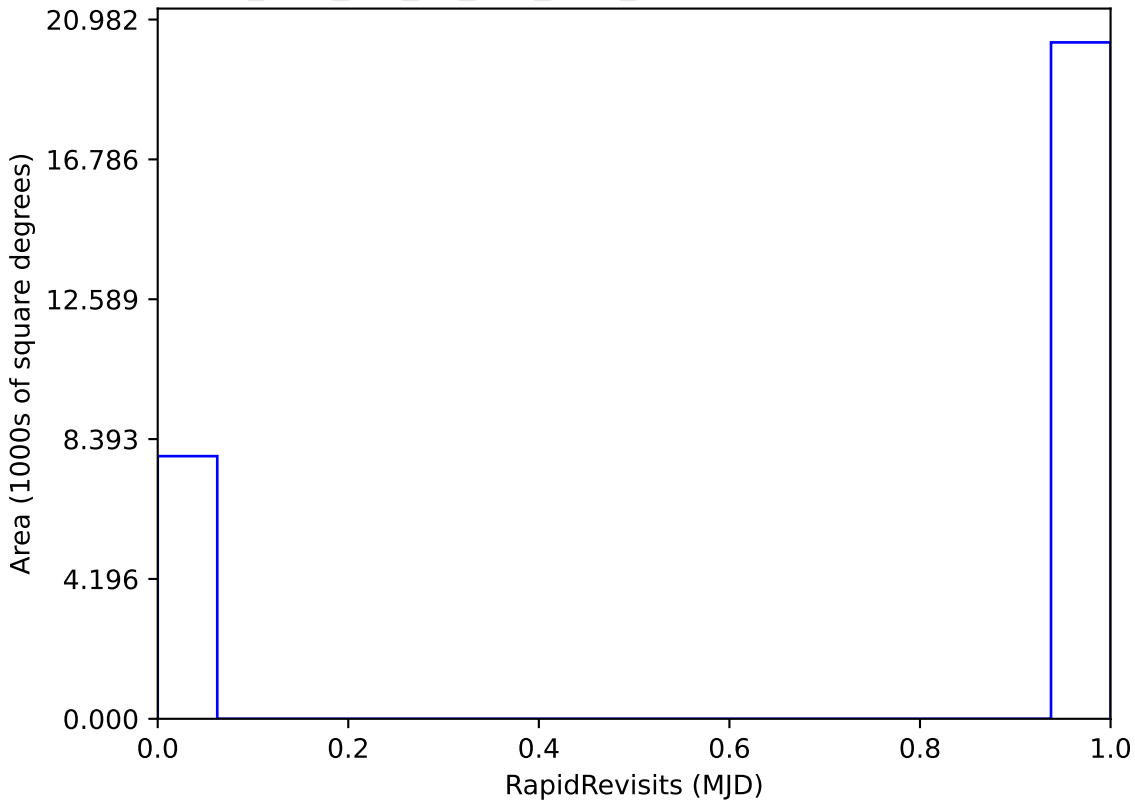
too_elab_r16_d3_griz_v3.4_10yrs All sky: RapidRevisits
