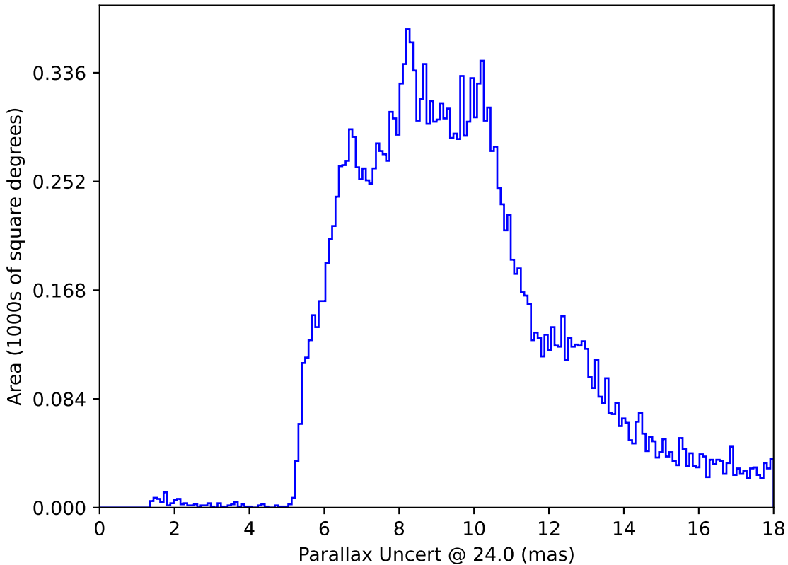
too_elab_r16_d3_griz_v3.4_10yrs All sky: Parallax Uncert @ 24.0
