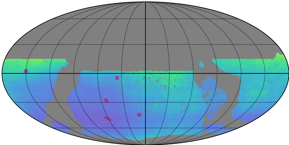
too_elab_r16_d3_griz_v3.4_10yrs WFD: Parallax Uncert @ 22.4
