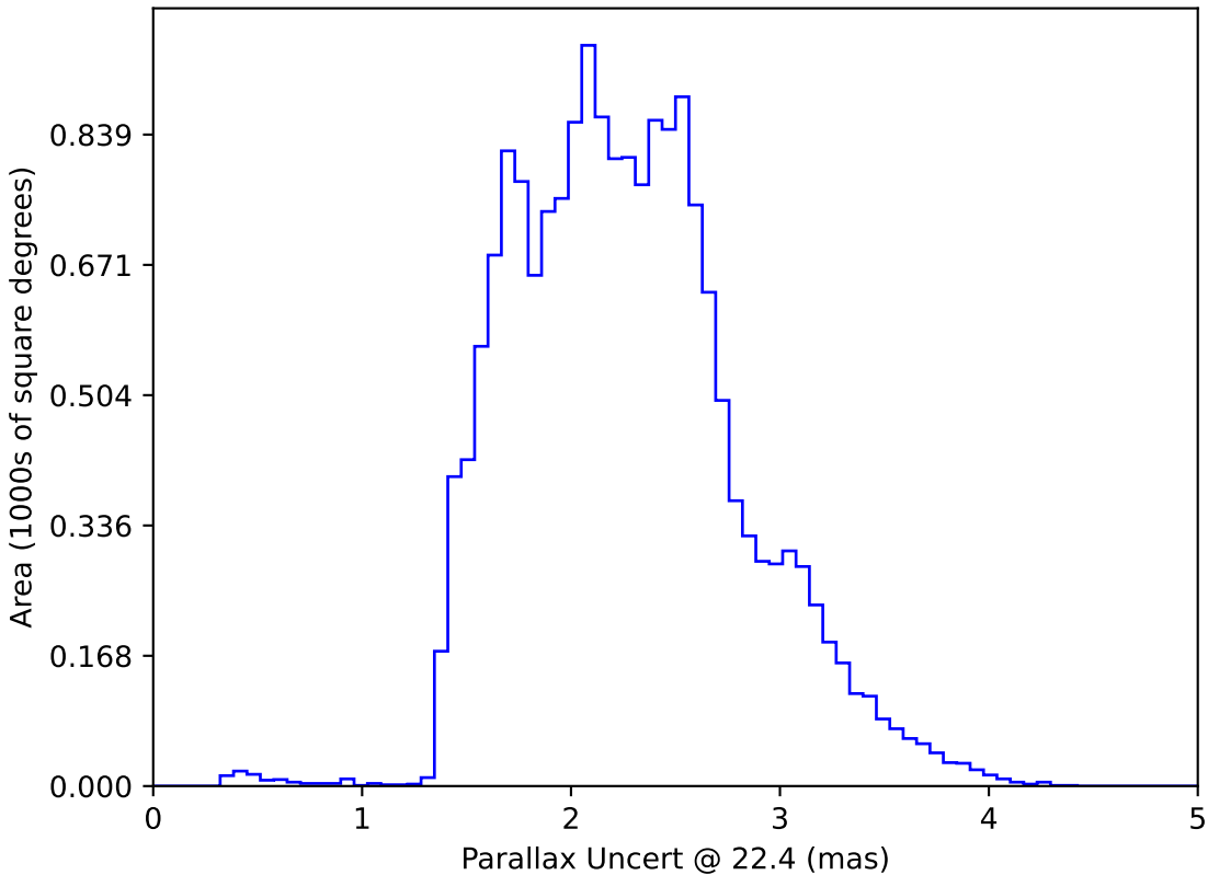
too_elab_r16_d3_griz_v3.4_10yrs WFD: Parallax Uncert @ 22.4
