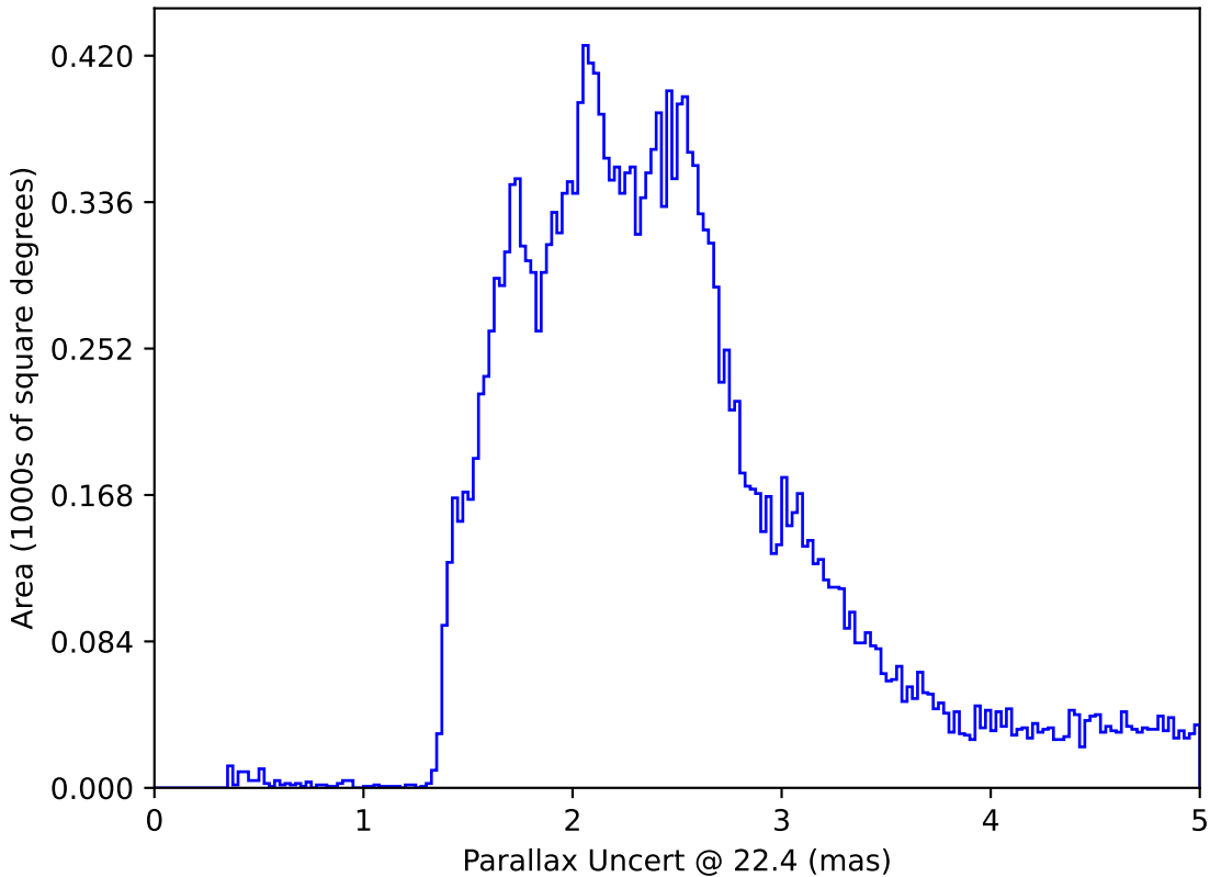
too_elab_r16_d3_griz_v3.4_10yrs All sky: Parallax Uncert @ 22.4
