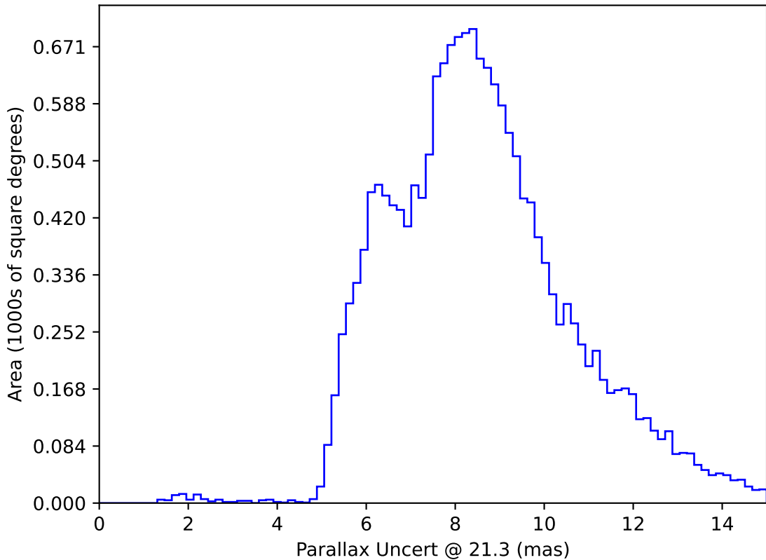
too_elab_r16_d3_griz_v3.4_10yrs WFD y band only: Parallax Uncert @ 21.3
