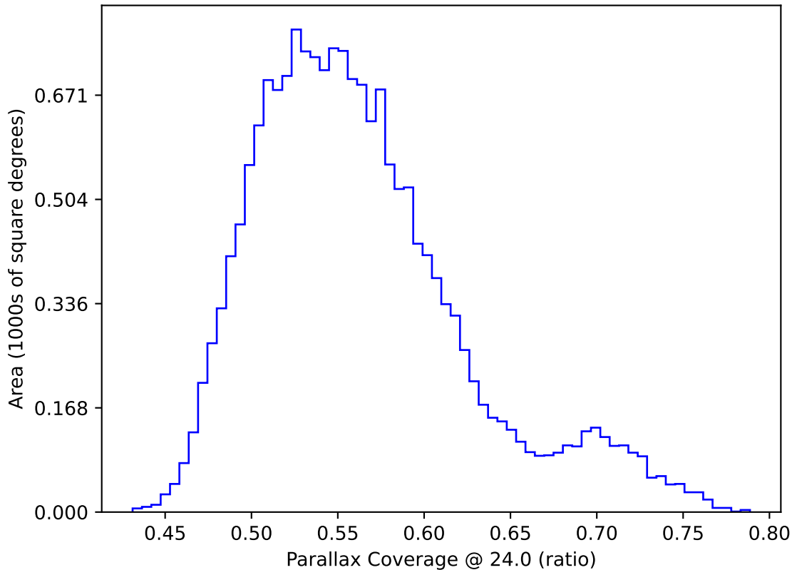
too_elab_r16_d3_griz_v3.4_10yrs WFD: Parallax Coverage @ 24.0
