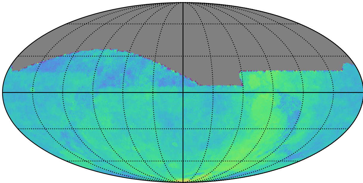
too_elab_r16_d3_griz_v3.4_10yrs All sky: Parallax Coverage @ 24.0
