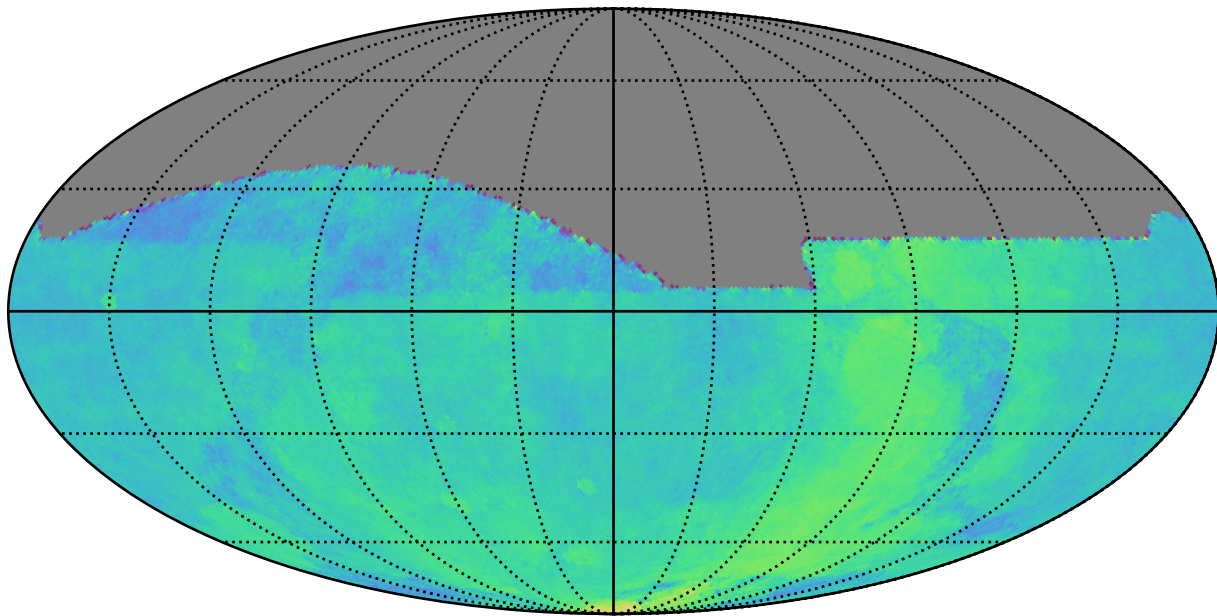
too_elab_r16_d3_griz_v3.4_10yrs All sky: Parallax Coverage @ 22.4
