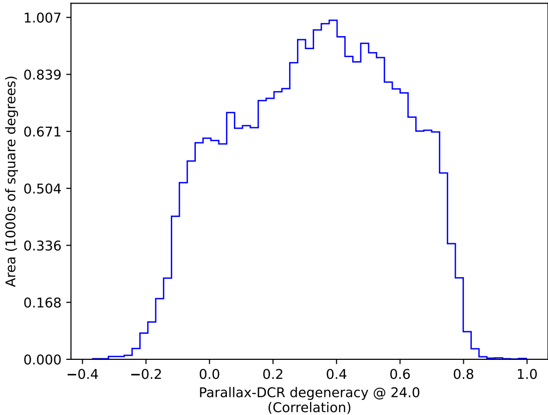
too_elab_r16_d3_griz_v3.4_10yrs All sky: Parallax-DCR degeneracy @ 24.0
