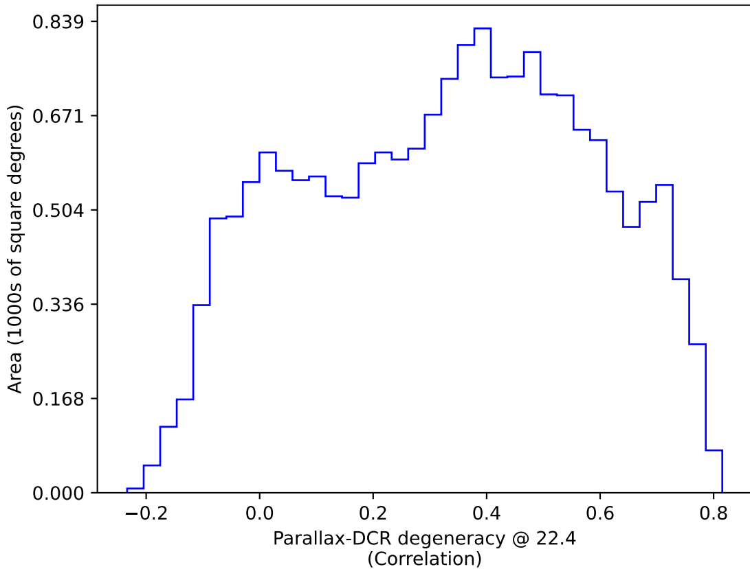
too_elab_r16_d3_griz_v3.4_10yrs WFD: Parallax-DCR degeneracy @ 22.4
