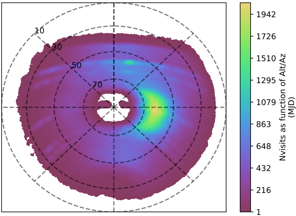
too_elab_r16_d3_griz_v3.4_10yrs y band: Nvisits as function of Alt/Az
