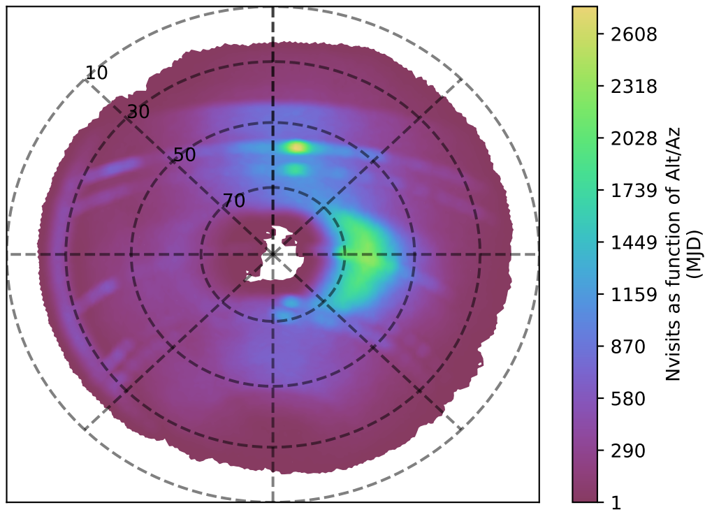
too_elab_r16_d3_griz_v3.4_10yrs r band: Nvisits as function of Alt/Az
