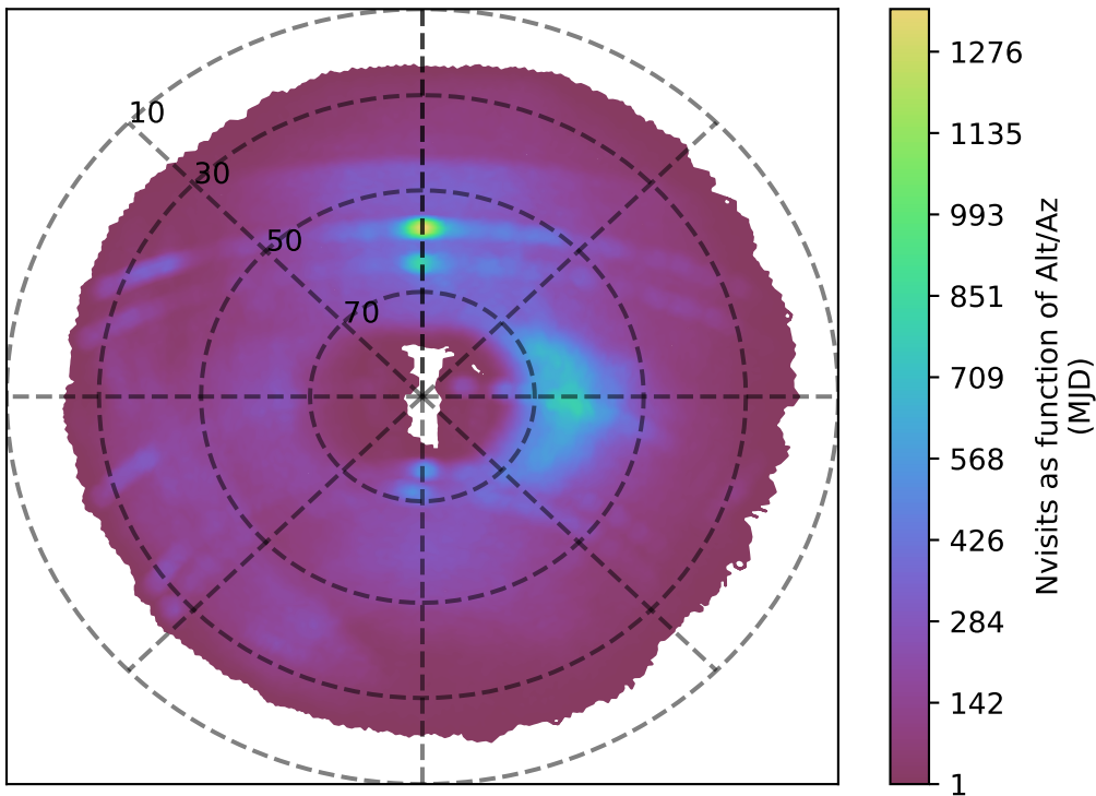
too_elab_r16_d3_griz_v3.4_10yrs g band: Nvisits as function of Alt/Az
