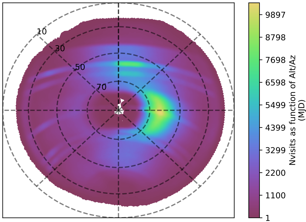
too_elab_r16_d3_griz_v3.4_10yrs all bands: Nvisits as function of Alt/Az
