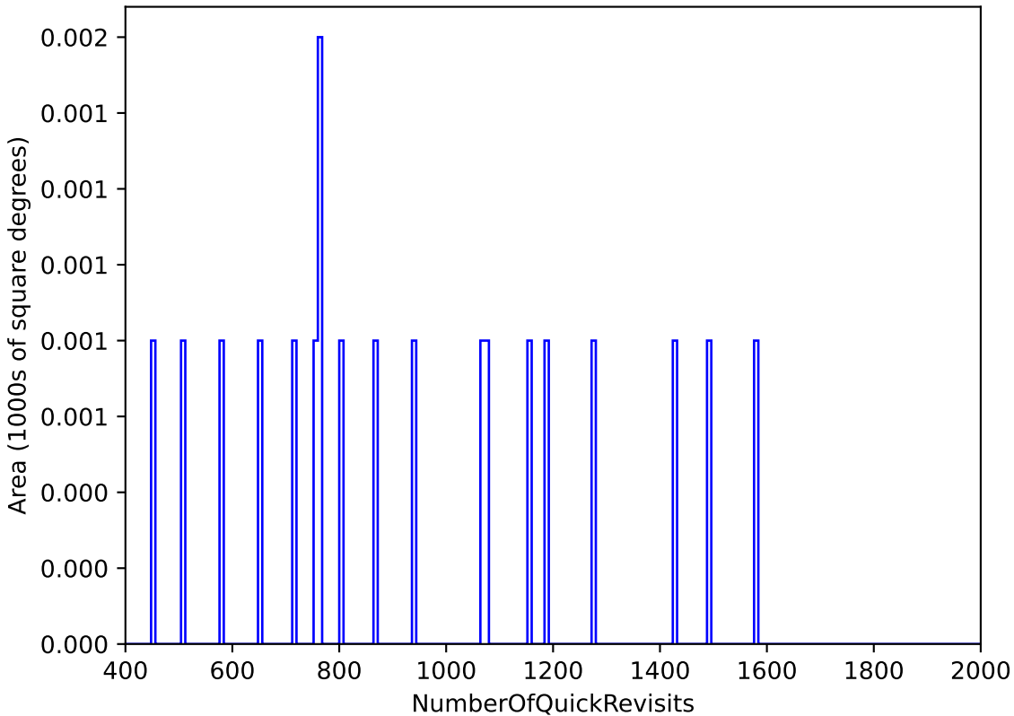
too_elab_r16_d3_griz_v3.4_10yrs All sky: NumberOfQuickRevisits
