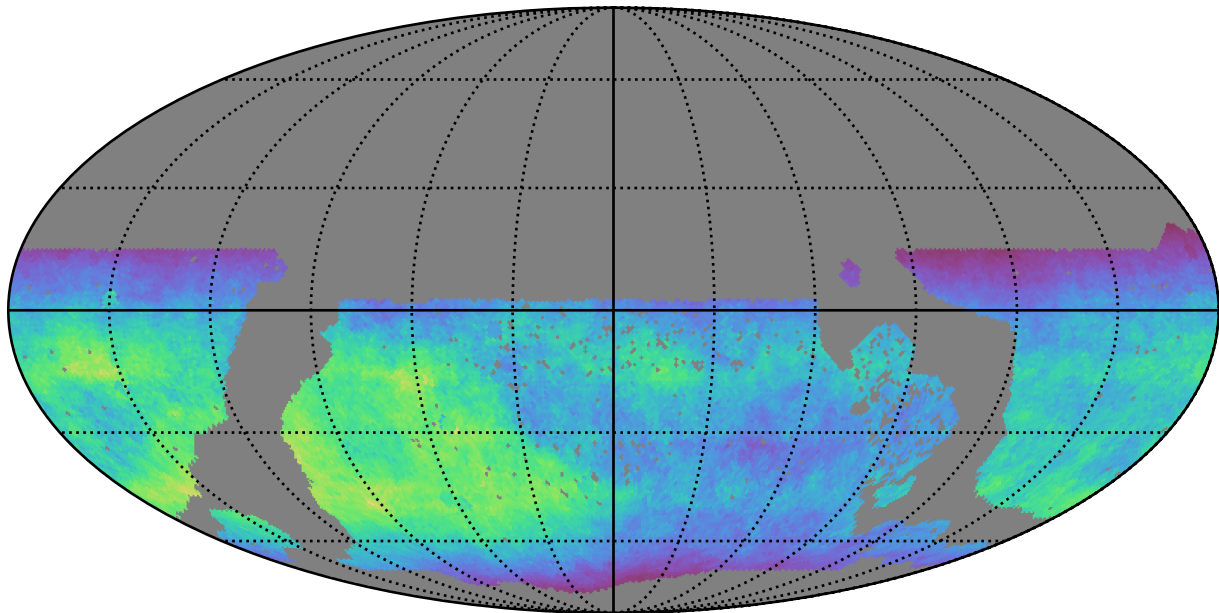
too_elab_r16_d3_griz_v3.4_10yrs WFD z band: Normalized Teff
