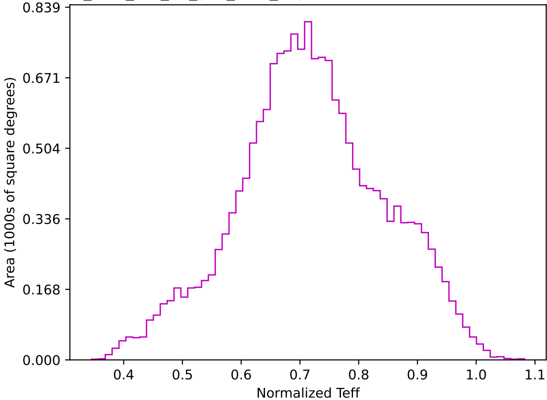
too_elab_r16_d3_griz_v3.4_10yrs WFD z band: Normalized Teff
