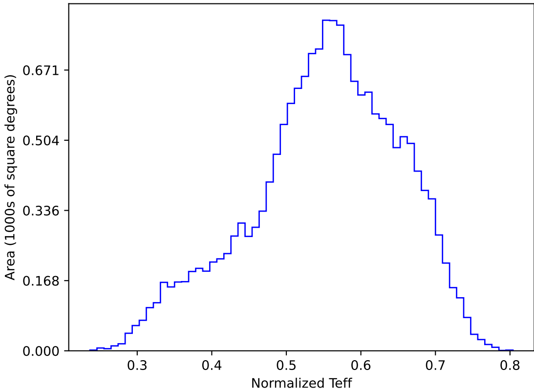
too_elab_r16_d3_griz_v3.4_10yrs WFD y band: Normalized Teff
