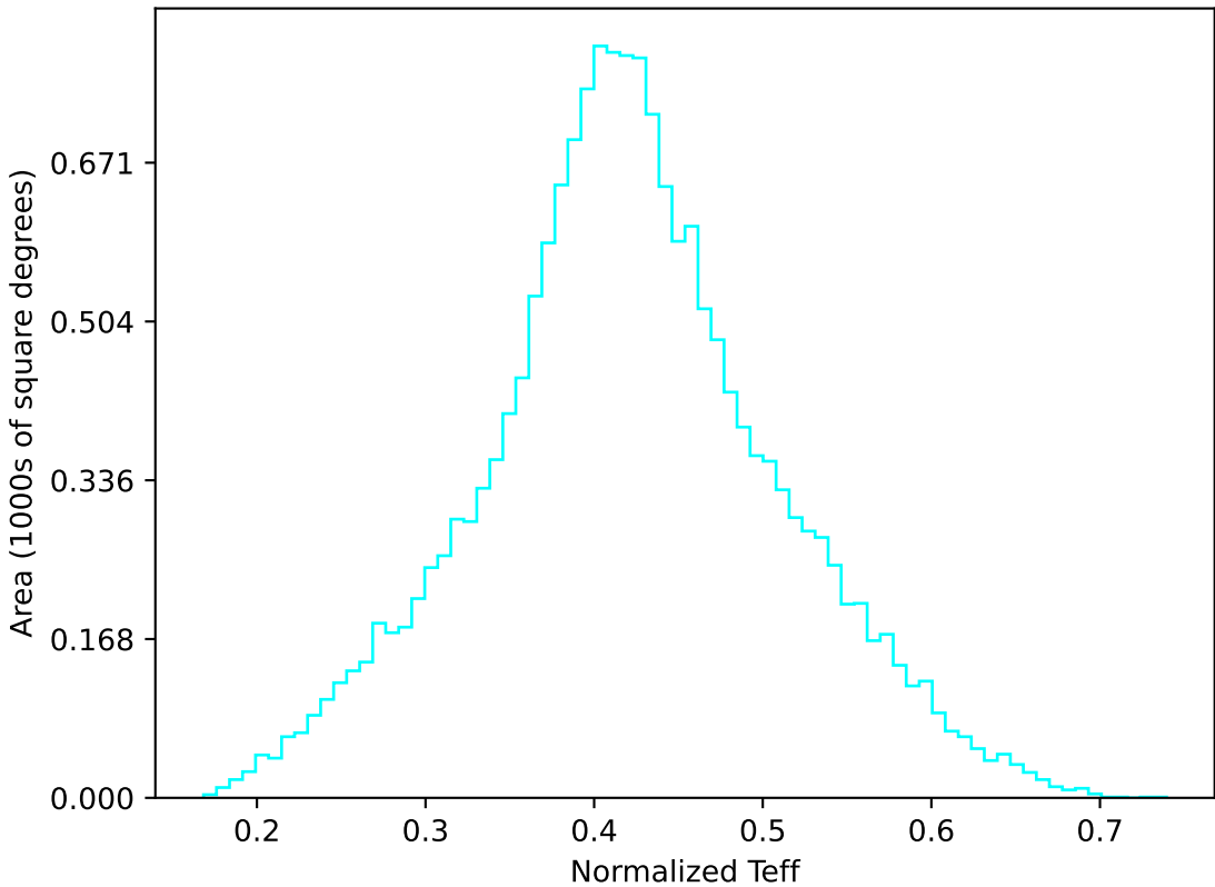
too_elab_r16_d3_griz_v3.4_10yrs WFD u band: Normalized Teff
