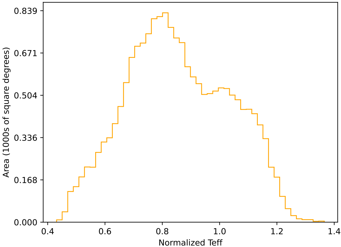
too_elab_r16_d3_griz_v3.4_10yrs WFD r band: Normalized Teff
