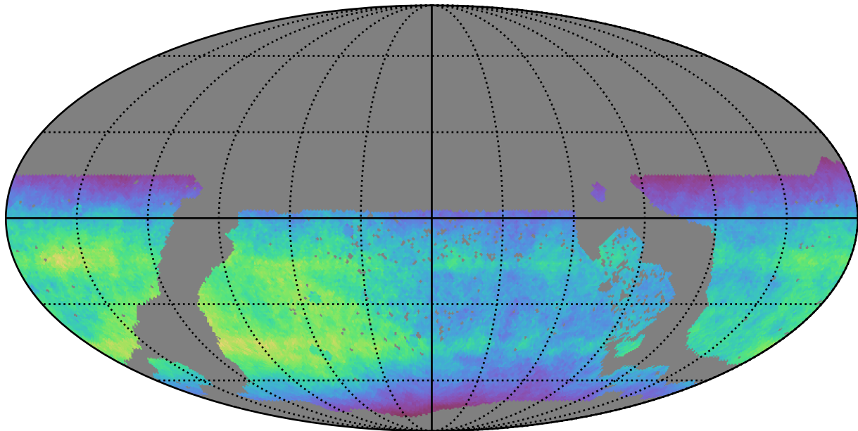
too_elab_r16_d3_griz_v3.4_10yrs WFD i band: Normalized Teff
