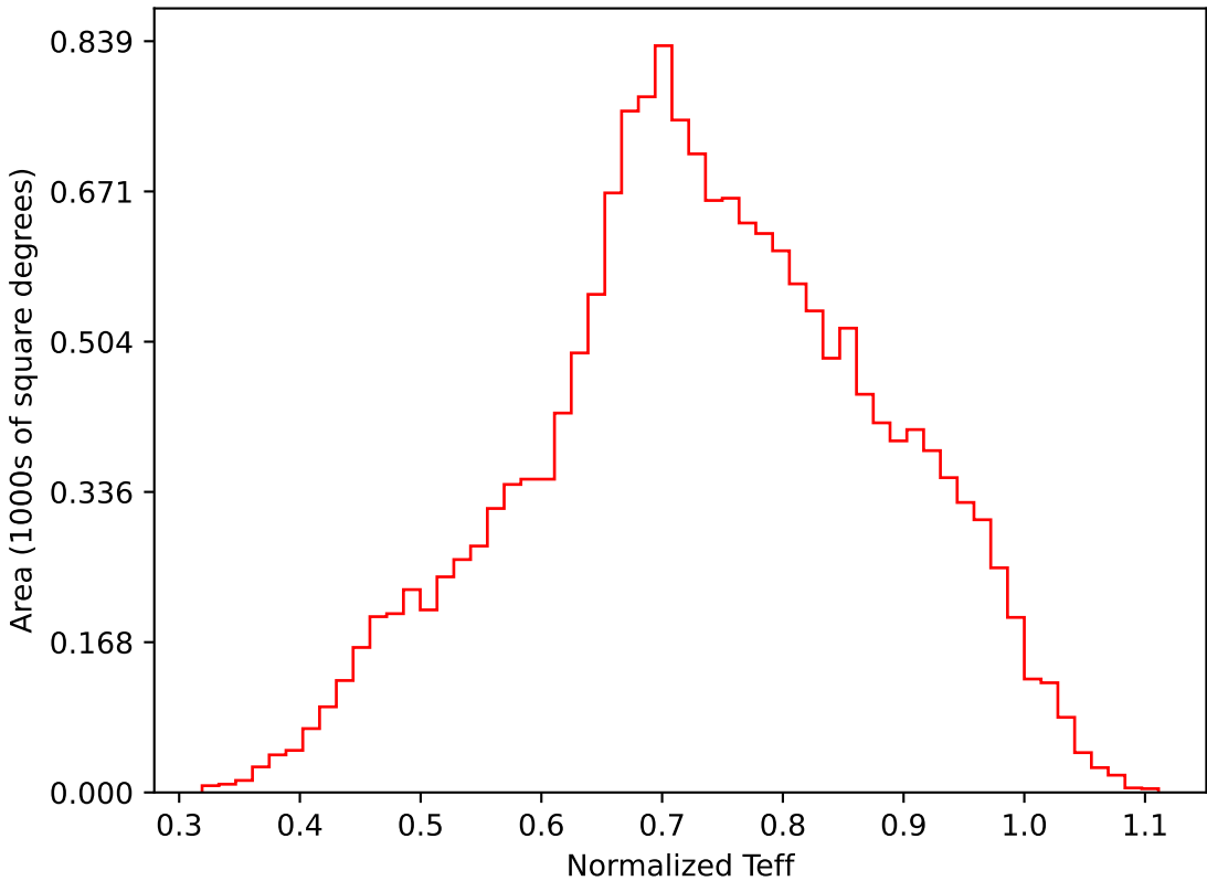
too_elab_r16_d3_griz_v3.4_10yrs WFD i band: Normalized Teff
