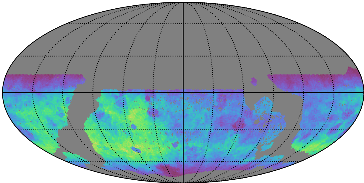
too_elab_r16_d3_griz_v3.4_10yrs WFD g band: Normalized Teff
