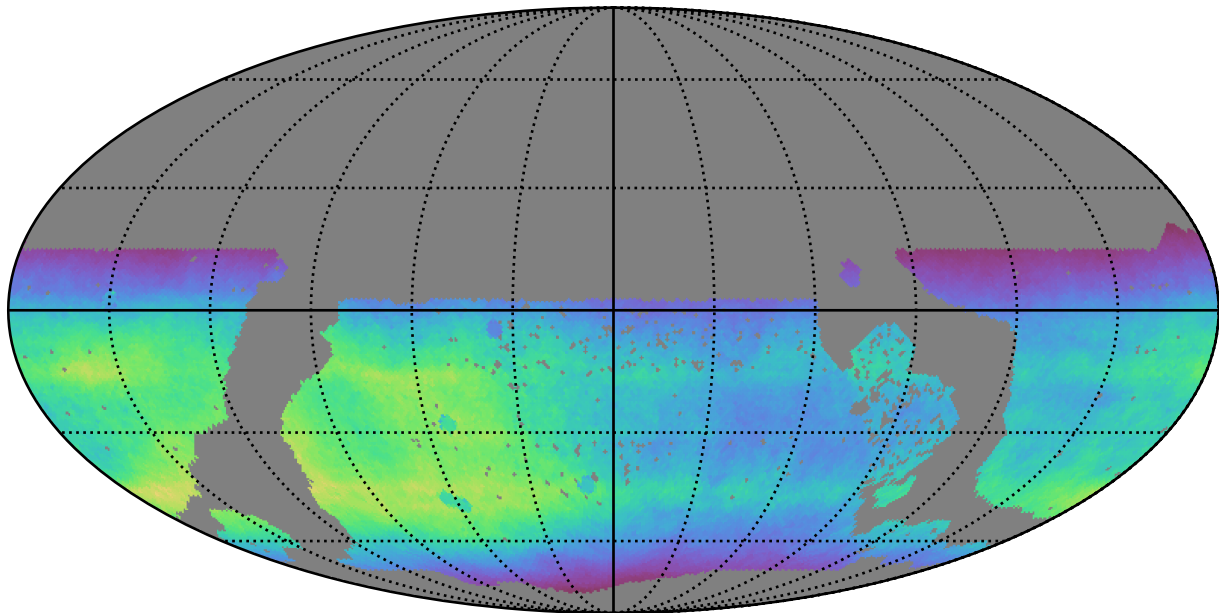
too_elab_r16_d3_griz_v3.4_10yrs WFD all bands: Normalized Teff
