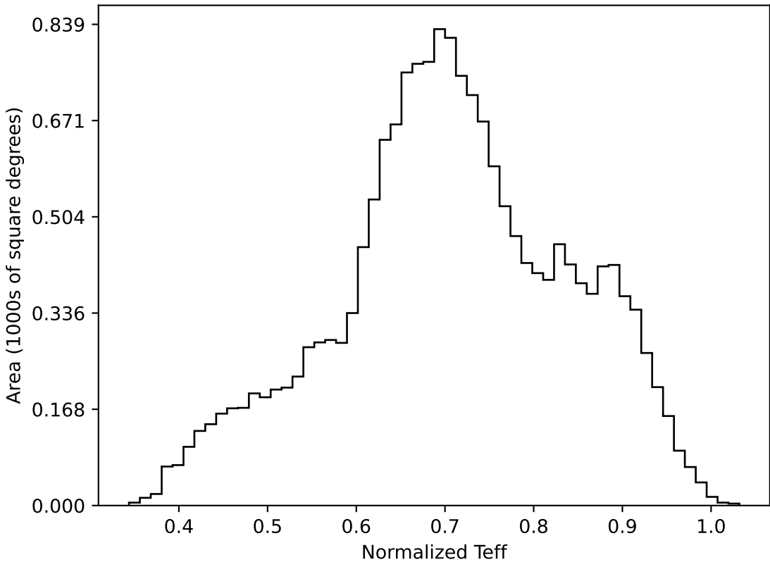
too_elab_r16_d3_griz_v3.4_10yrs WFD all bands: Normalized Teff
