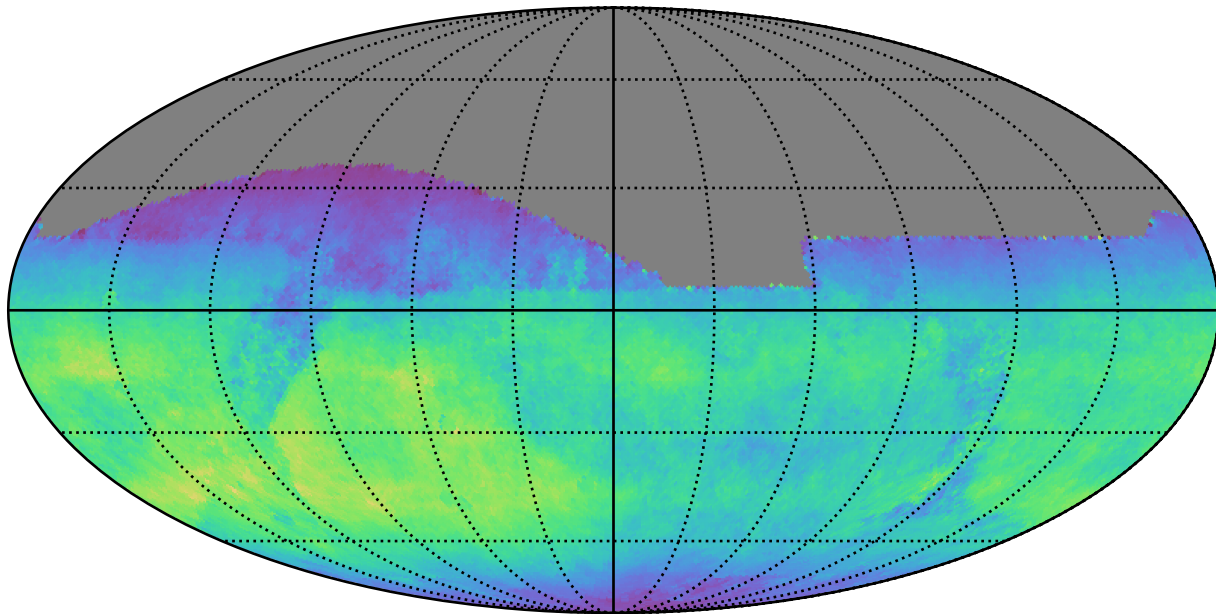
too_elab_r16_d3_griz_v3.4_10yrs All sky z band: Normalized Teff
