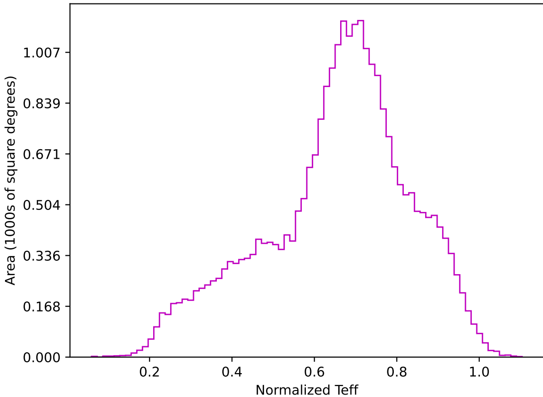
too_elab_r16_d3_griz_v3.4_10yrs All sky z band: Normalized Teff
