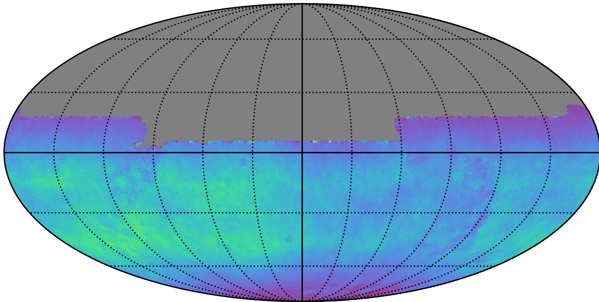
too_elab_r16_d3_griz_v3.4_10yrs All sky y band: Normalized Teff
