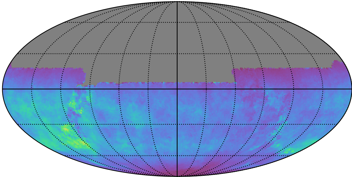
too_elab_r16_d3_griz_v3.4_10yrs All sky u band: Normalized Teff
