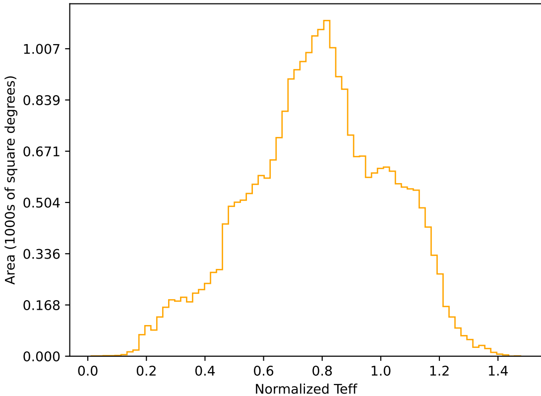
too_elab_r16_d3_griz_v3.4_10yrs All sky r band: Normalized Teff
