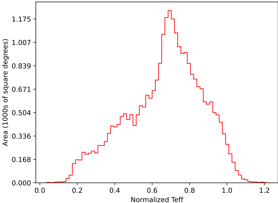
too_elab_r16_d3_griz_v3.4_10yrs All sky i band: Normalized Teff
