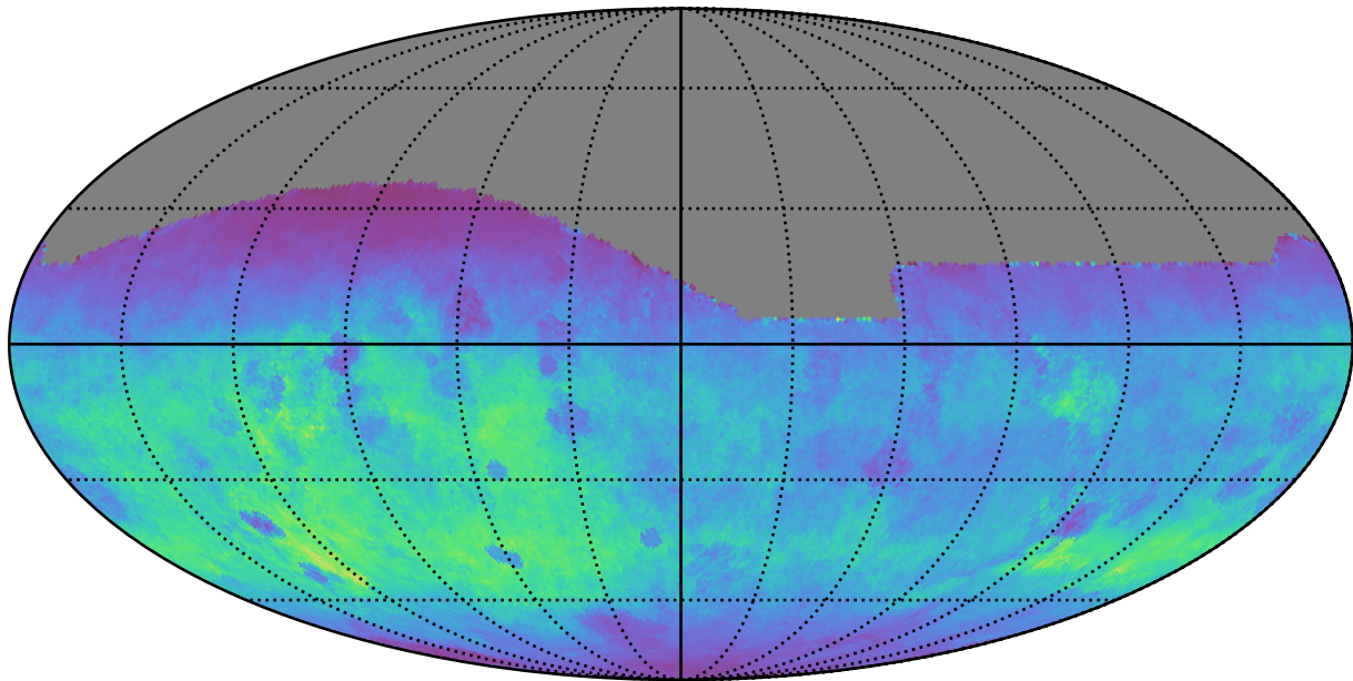
too_elab_r16_d3_griz_v3.4_10yrs All sky g band: Normalized Teff
