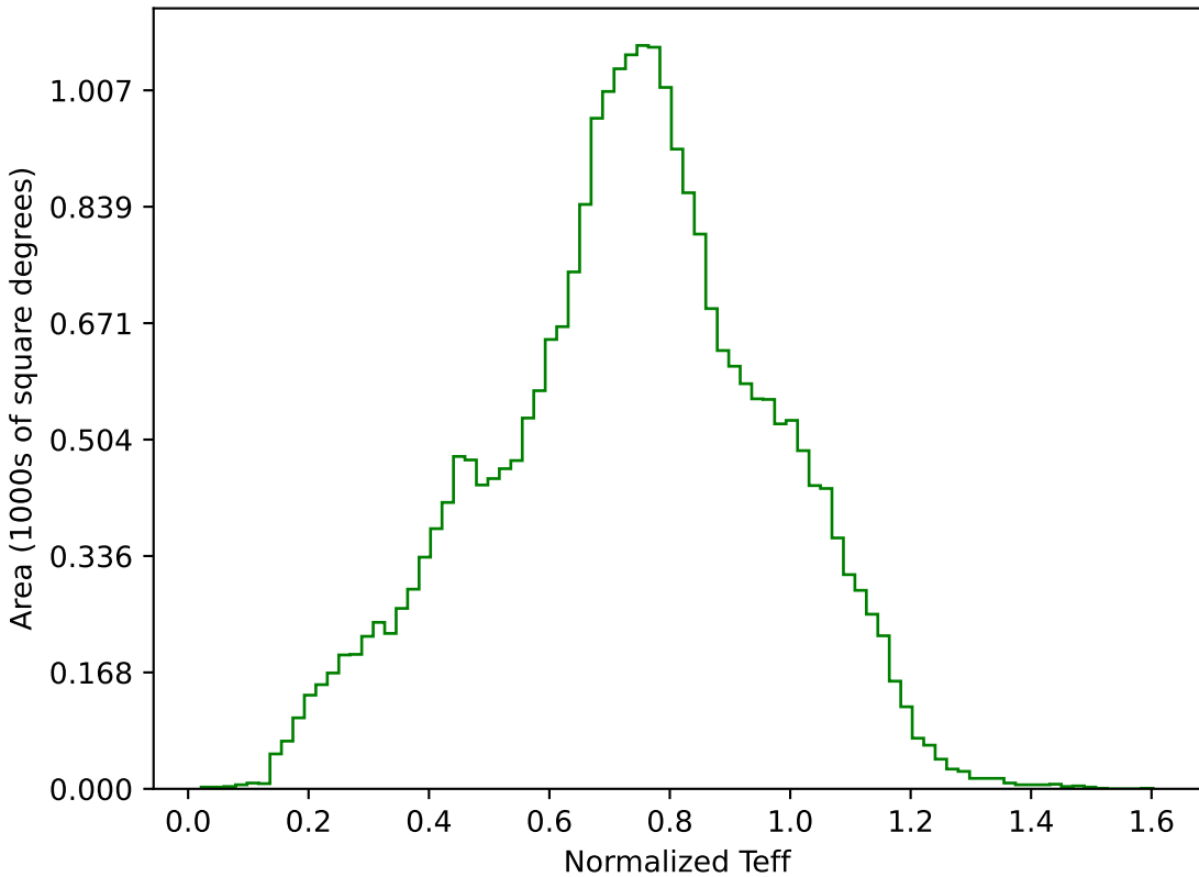
too_elab_r16_d3_griz_v3.4_10yrs All sky g band: Normalized Teff
