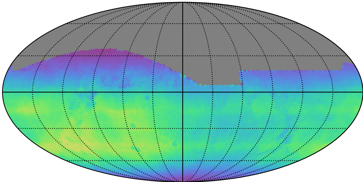
too_elab_r16_d3_griz_v3.4_10yrs All sky all bands: Normalized Teff
