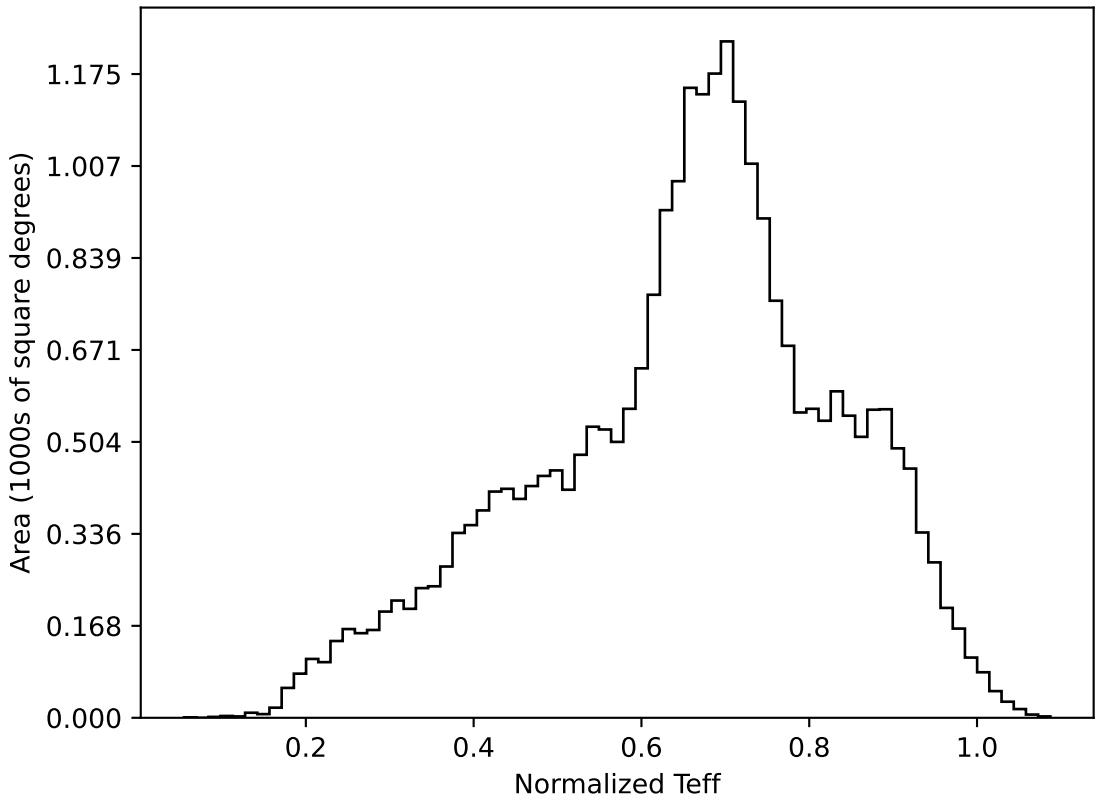
too_elab_r16_d3_griz_v3.4_10yrs All sky all bands: Normalized Teff
