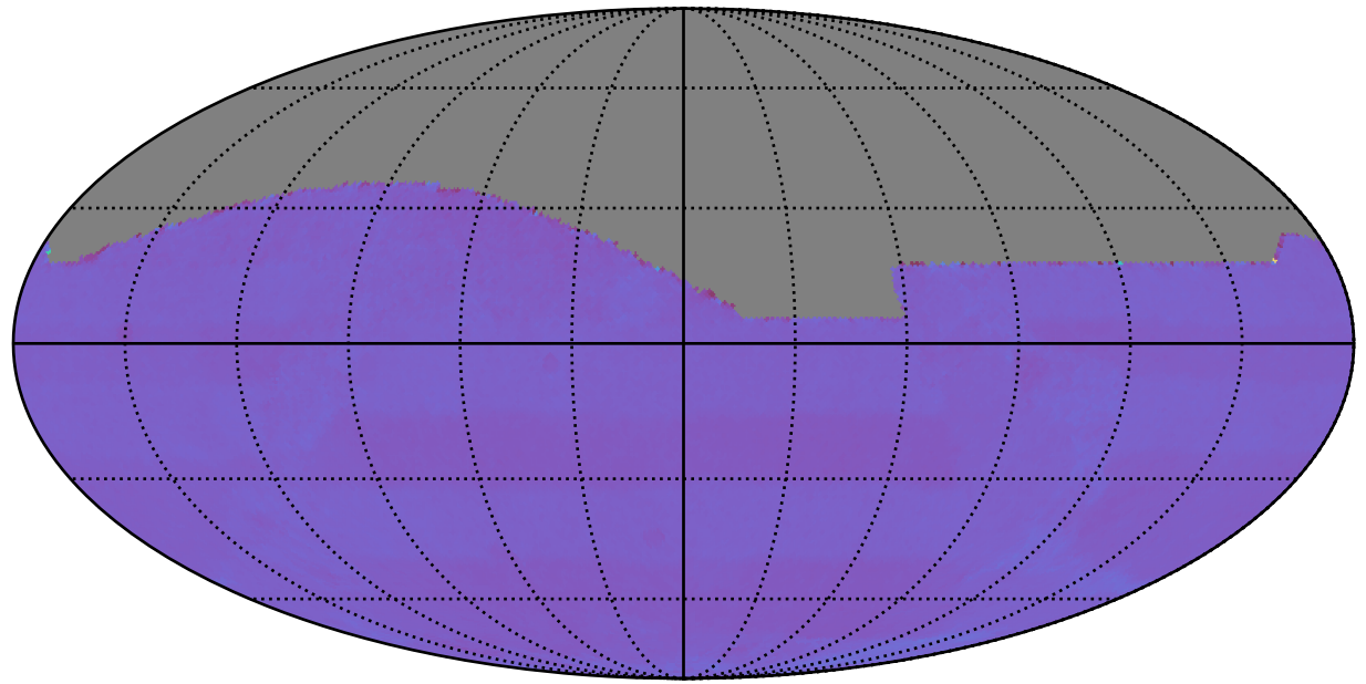
too_elab_r16_d3_griz_v3.4_10yrs All sky: Normalized Proper Motion Uncert @ 20.5
