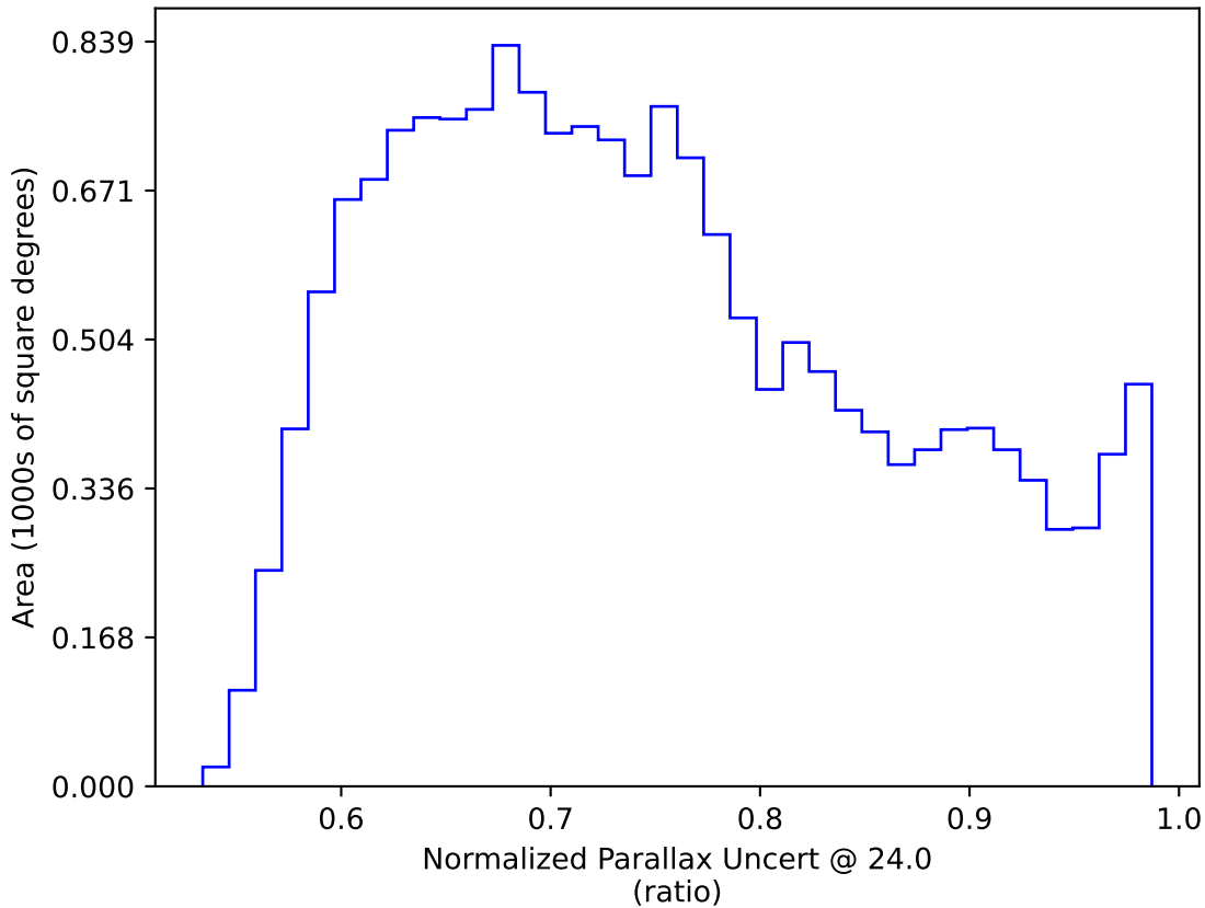
too_elab_r16_d3_griz_v3.4_10yrs WFD: Normalized Parallax Uncert @ 24.0
