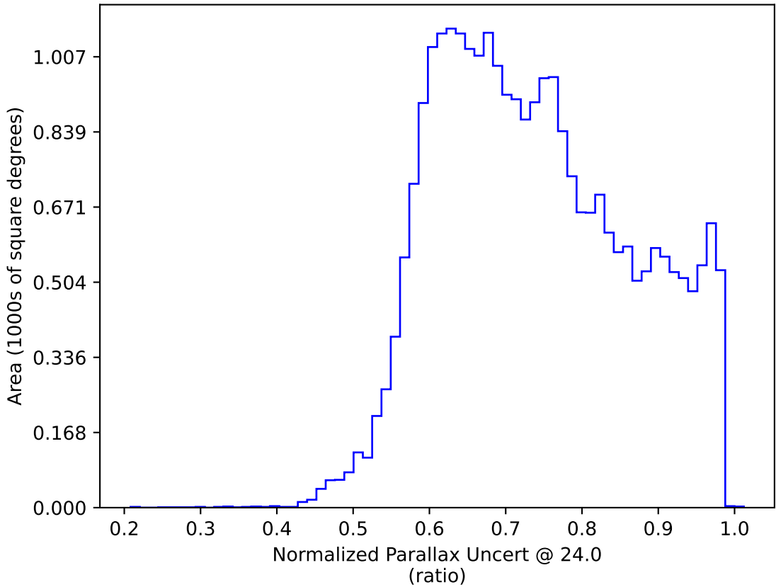
too_elab_r16_d3_griz_v3.4_10yrs All sky: Normalized Parallax Uncert @ 24.0
