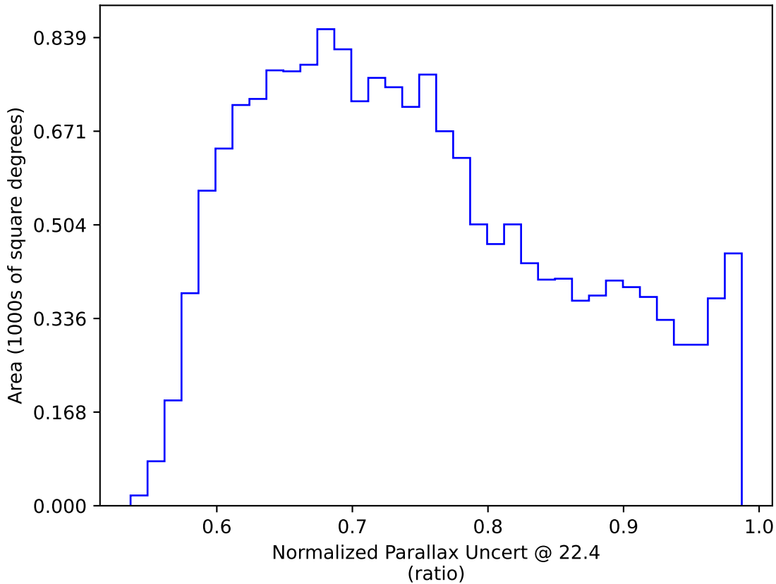
too_elab_r16_d3_griz_v3.4_10yrs WFD: Normalized Parallax Uncert @ 22.4
