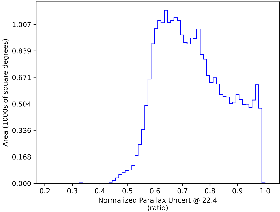
too_elab_r16_d3_griz_v3.4_10yrs All sky: Normalized Parallax Uncert @ 22.4
