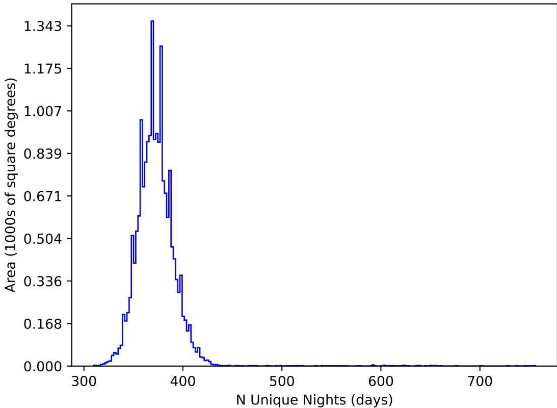
too_elab_r16_d3_griz_v3.4_10yrs WFD all bands: N Unique Nights
