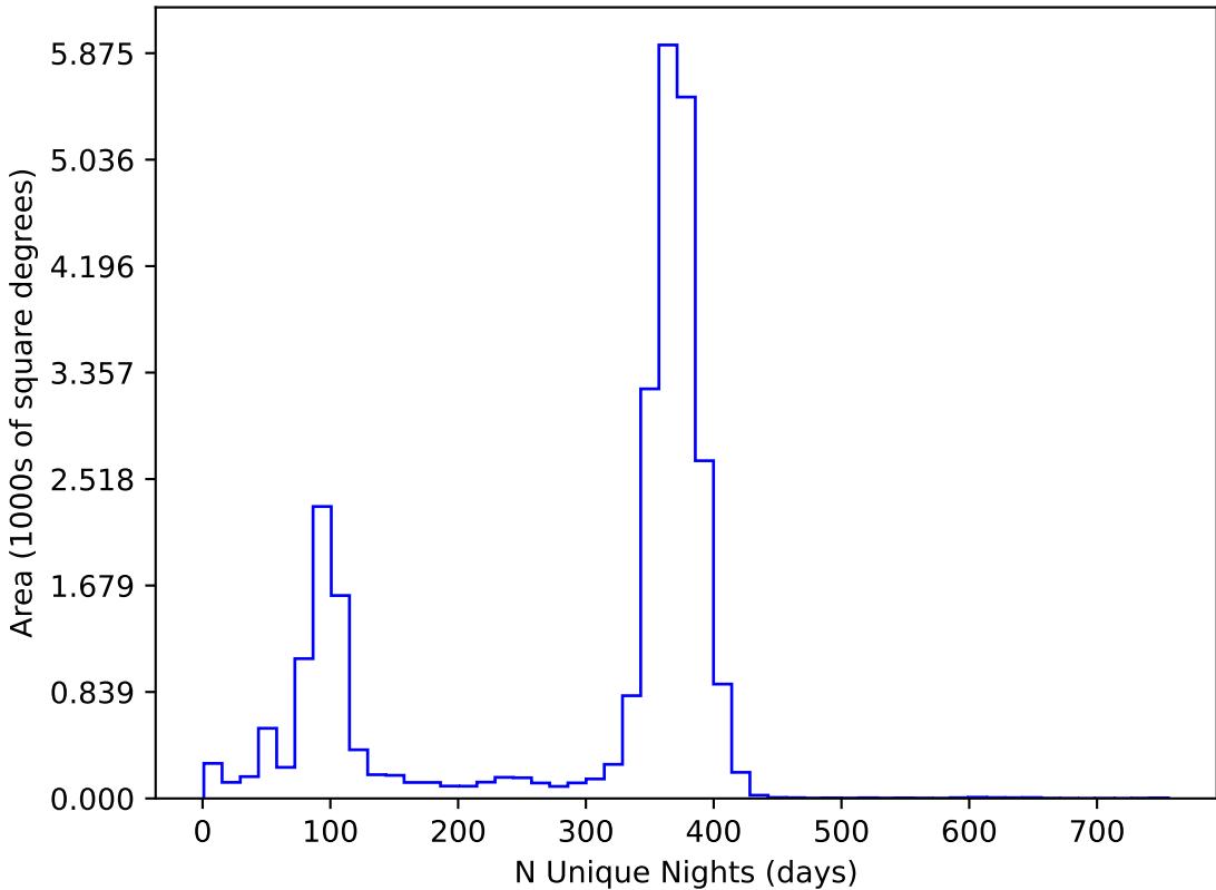
too_elab_r16_d3_griz_v3.4_10yrs All sky all bands: N Unique Nights
