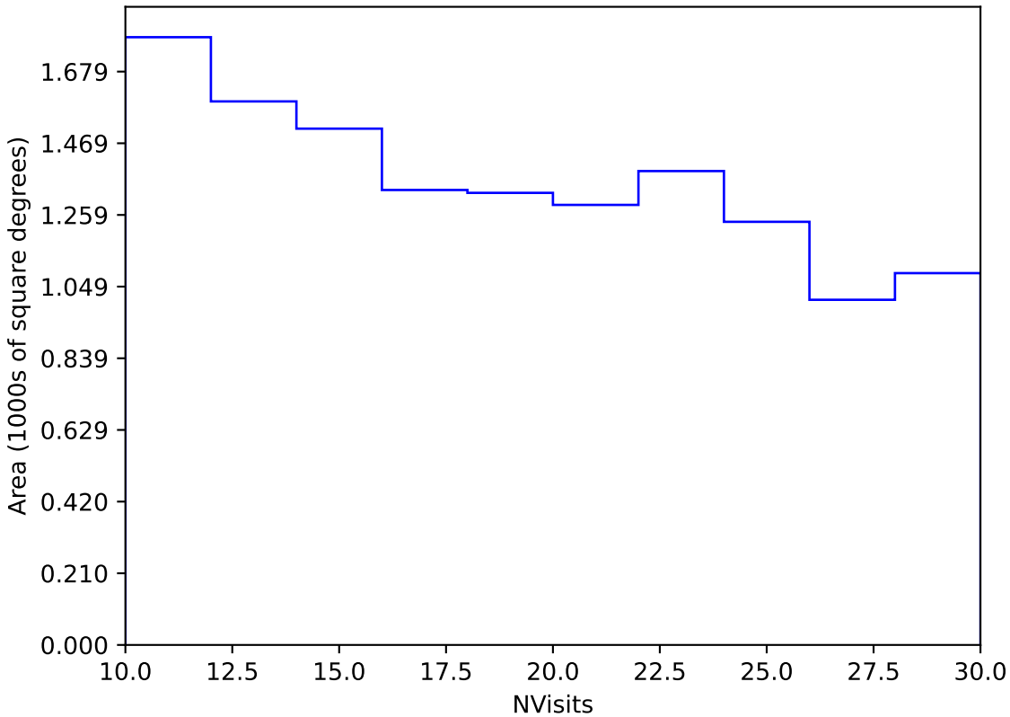
too_elab_r16_d3_griz_v3.4_10yrs Yr 3-4 y band: NVisits
