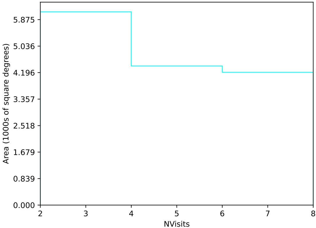
too_elab_r16_d3_griz_v3.4_10yrs Yr 3-4 u band: NVisits
