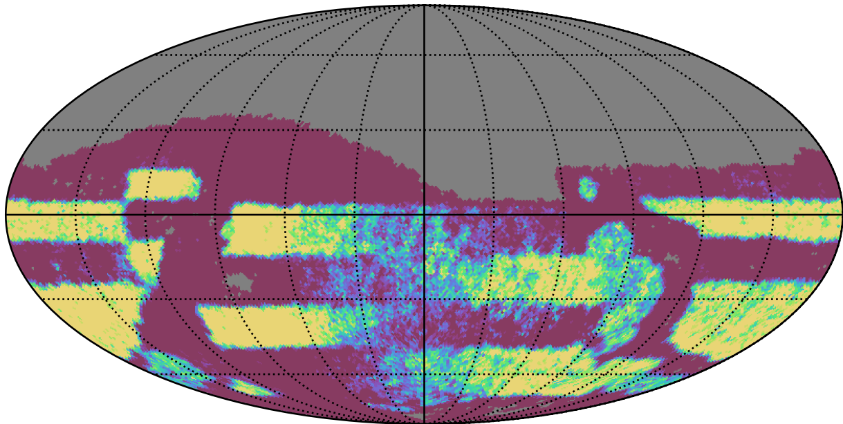
too_elab_r16_d3_griz_v3.4_10yrs Yr 3-4 r band: NVisits
