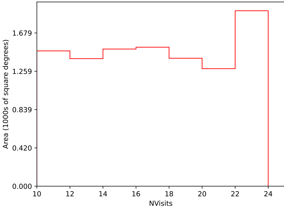
too_elab_r16_d3_griz_v3.4_10yrs Yr 3-4 i band: NVisits
